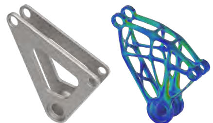
Original bellcrank
