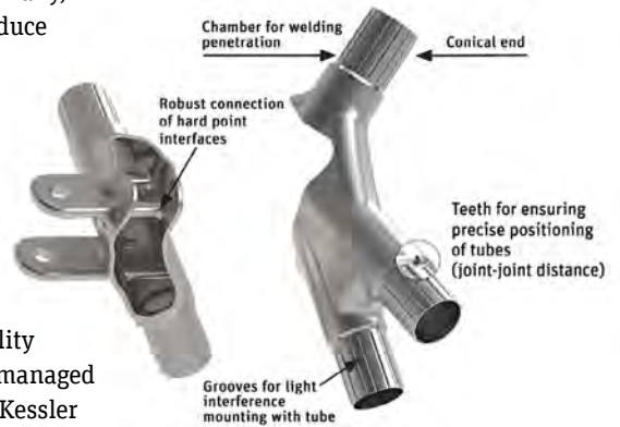
3D-printed joint for greater strength and torsional stiffness
