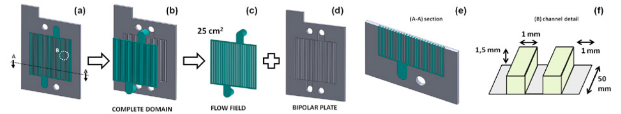
Geometry for the simulation model: (a) bipolar plate with the flow distribution channels; (b) complete domain; (c) parallel flow field; (d) bipolar plate; (e) section of the channels of the bipolar plate; (f) detailed dimensions of the channels
