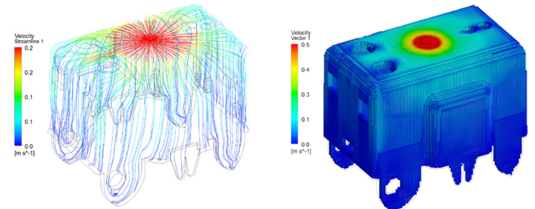
ANSYS Fluent mold-filling simulation predicts weld lines.
