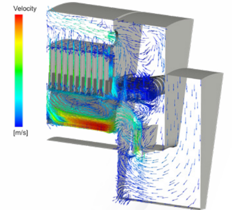
ANSYS Fluent simulation of the velocity profile of a generator helps to ensure adequate cooling airflow.
