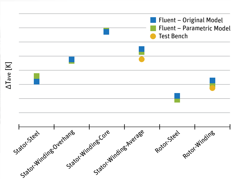
Temperatures obtained using the old workflow (starting from design drawing). The new workflow (parametrized model) and the measurements from the test bench were in agreement.
