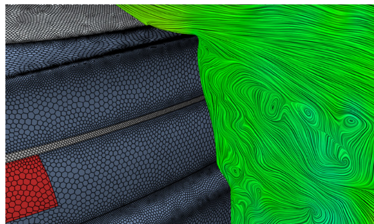
Mosaic-enabled mesh was used to capture details of turbulent flow around the rear of this car.
