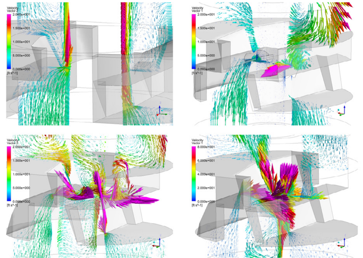
CFD flow fields with the ram closing on the pipe
