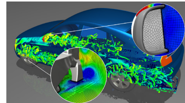
Detailed aerodynamics SBES simulation of DrivAer model shows details of Mosaic meshing and turbulent airflow around the wheel hub and the external side mirror.
