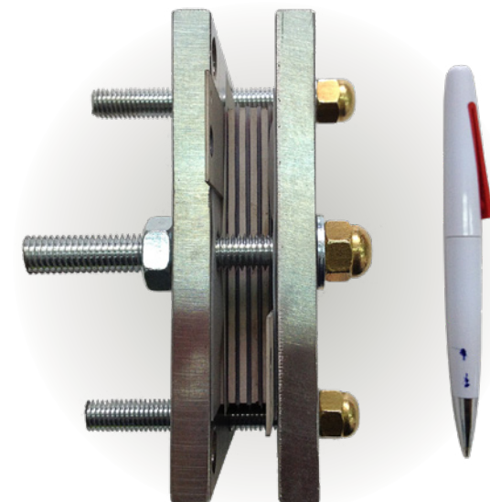
A PEM water electrolysis stack for hydrogen production with purity higher than 99.995%. The active area is 25 cm 2 and the maximum current density of 2,000 mA/cm 2 .
