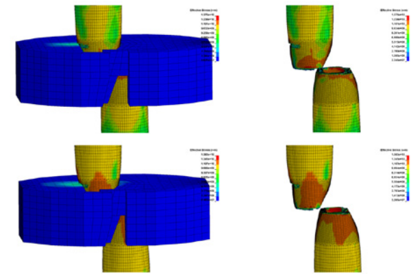
ANSYS Mechanical simulation showing stresses on the cut pipe
