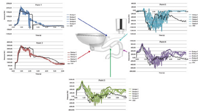
Pressure comparisons between CFD simulations and the physical toilet model — captured at different design points — proved to Roca engineers that they could rely on simulation.
