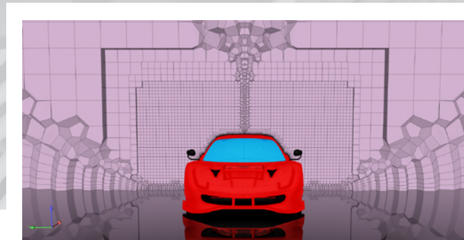
Mosaic-enabled meshing
