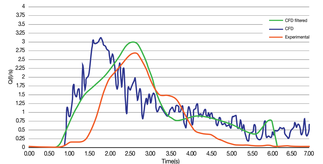
Flow rate comparison between an ANSYS simulation and real-world results from a physical model demonstrates the accuracy of simulating toilet performance via ANSYS solutions.
