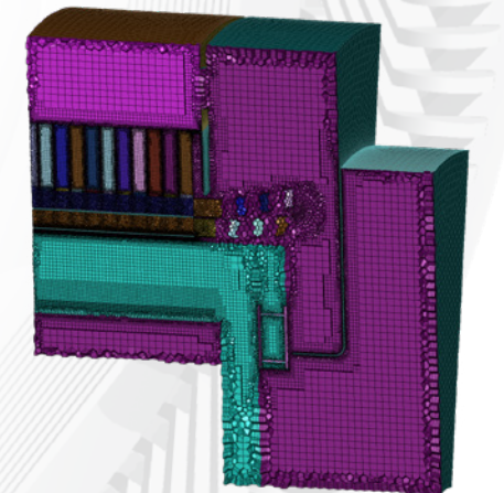
Mosaic-enabled poly-hexcore mesh
