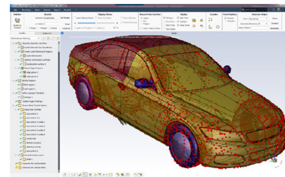
ANSYS Fluent's new fault-tolerant workflow simplifies CFD analysis of non-watertight CAD models. Geometry courtesy of Technical University of Munich (TUM)
