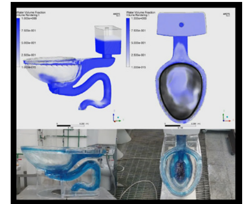
By first constructing a physical toilet model, Roca engineers were able to compare and verify the results of their early simulations — giving them the confidence they needed to eliminate some physical testing.
