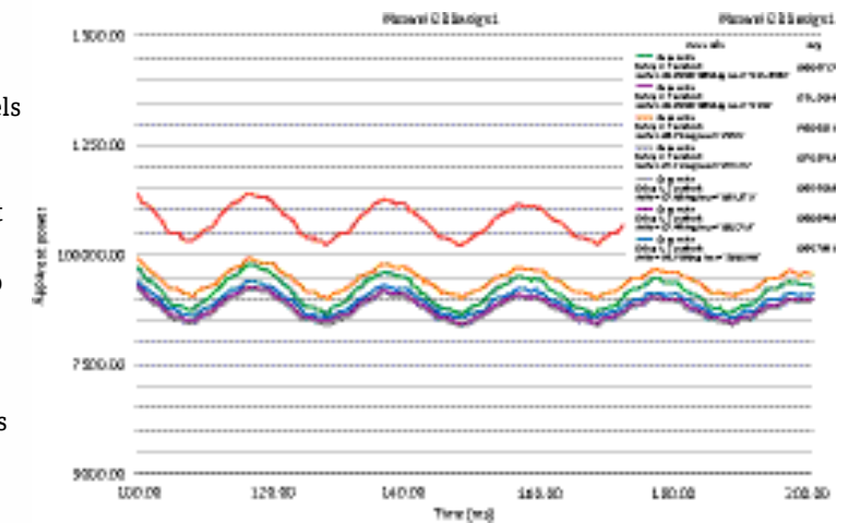
ANSYS Maxwell simulation for apparent power using the new workflow
