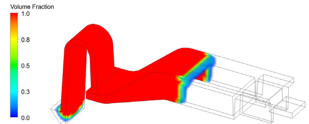
Volume fraction of plastic filling the mold
