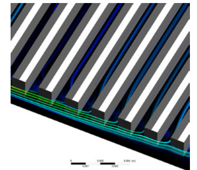
Streamlines at the closest part of the bipolar plate to the channel inflow at 500 mA/cm 2 and 100 mL/min. In some channels, when the flow rate is high, vorticity phenomena may occur. This limits the water flow in each channel so that the hydrogen generated in the cell accumulates, reducing the efficiency of the process.
