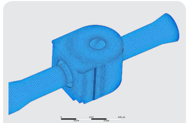
Overall volume mesh for CFD simulation
