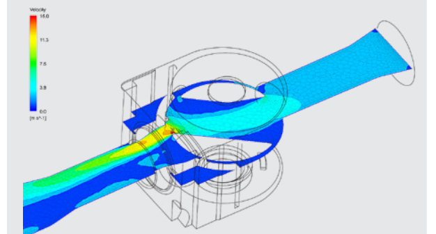
Velocity contour plot of valve at partially opened position
